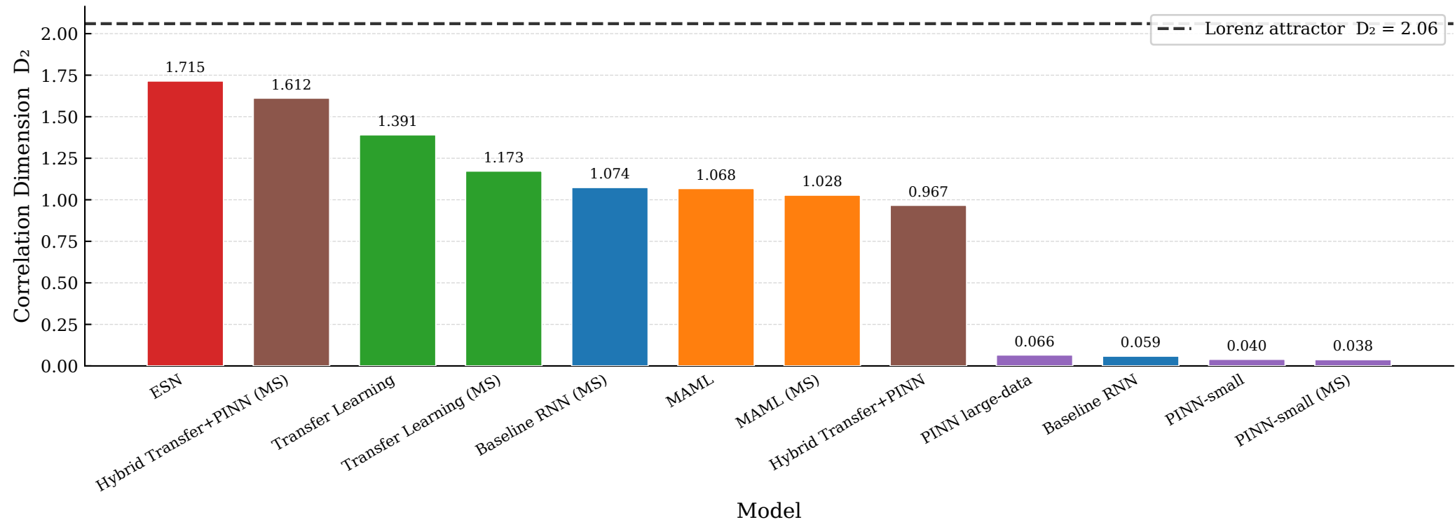
Lorenz — Correlation Dimension D_2 Closer to reference line = better attractor reconstruction
